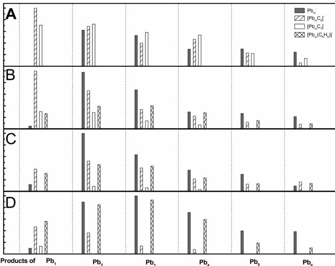
Figure 5. The statistical relative intensities of four representative product series ( Pb_m^- , [Pb_m C_4]^- , [Pb_m C_7]^- , and [Pb_m(C_6H_5)]^- ) when different concentrations of benzene (panel A, 0.625%; panel B, 0.313%; panel C, 0.15%; panel D, 0.075%) in total 400 kPa mixed gas were used.
